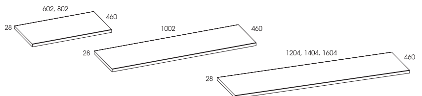
blaty 60, 80, 100, 120 / worktops 60, 80, 100 120,
