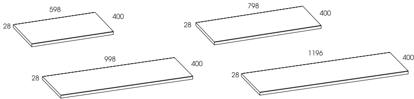
blaty 60, 80, 100, 120 worktops 60, 80, 100, 120
