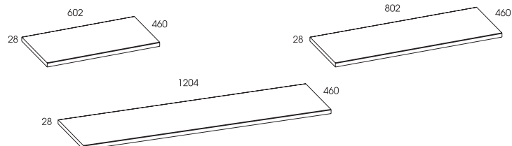
blaty 60, 80, 120 worktops 60, 80, 120
