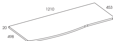
blat 81, 121, 161 worktop 81, 121, 161
